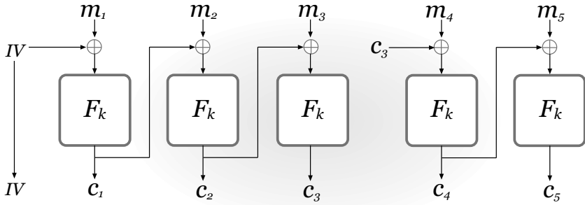
FIGURE 3.8: Chained CBC.
